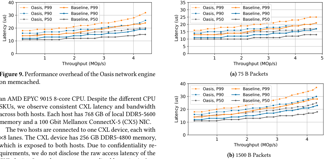
Figure 10. Performance overhead of the Oasis network engine on a UDP echo microbenchmark with different packet sizes.
