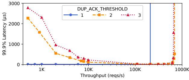
Figure 3: Tail latency vs throughput as a function of DUP_ACK_THRESHOLD while simulating 0.1% packet drop rate. Smaller DUP_ACK_THRESHOLD makes a significant tail latency reduction, especially at a lower load.
