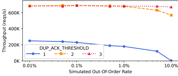
Figure 2: Throughput vs. packet out-of-order rate as a function of the DUP_ACK_THRESHOLD value. A smaller DUP_ACK_THRESHOLD results in reduced throughput, particularly when the packet out-of-order rate is high.
