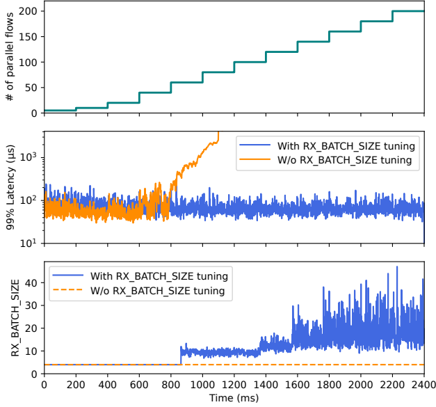
Figure 6: By tuning RX_BATCH_SIZE based on runtime OS signals, the system can maintain low tail latency even under dynamic workload conditions.
